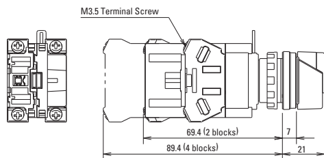
Full Voltage Model
