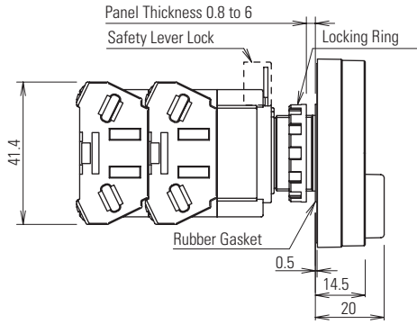
With Pilot Light
