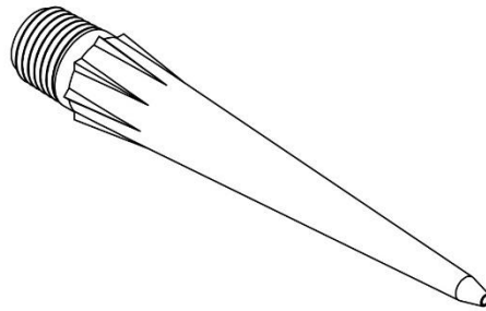
TS416-HO-HD-PK Precision Polypropylene Dispensing Nozzle, length 102 mm x Ø 1.6 mm, male threads 1/4" NPT
