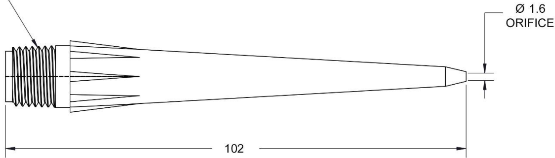
TS416-HO-HD-PK Precision Polypropylene Dispensing Nozzle, length 102 mm x Ø 1.6 mm, male threads 1/4" NPT
